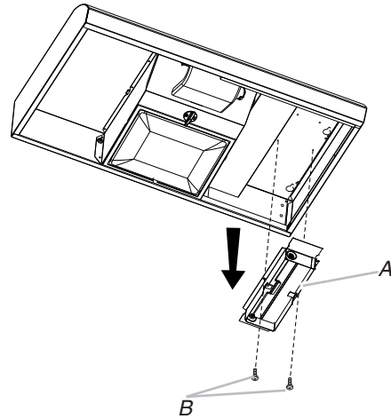
A. 3\frac{1}{4} " x 10" (8.3 x 25.4 cm) rectangular vent damper B. 3.5 x 9.5 mm screws
